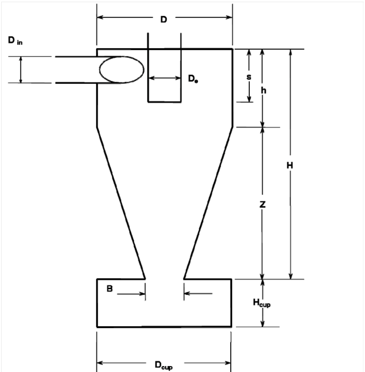
Figure 5. Design Specifications for Cyclone I (10 Micrometer)
