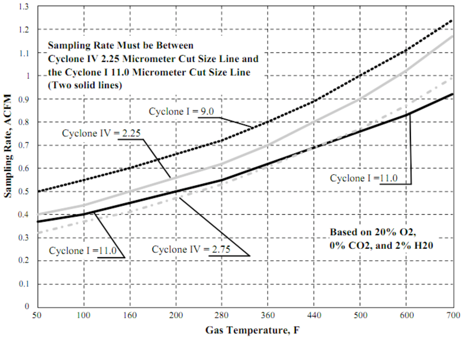
Figure 10. Acceptable Sampling Rate for Combined Cyclone Heads
