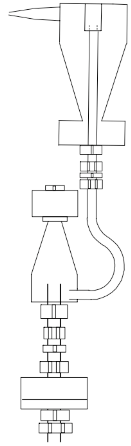
Figure 2. Combined Cyclone Sampling Head
