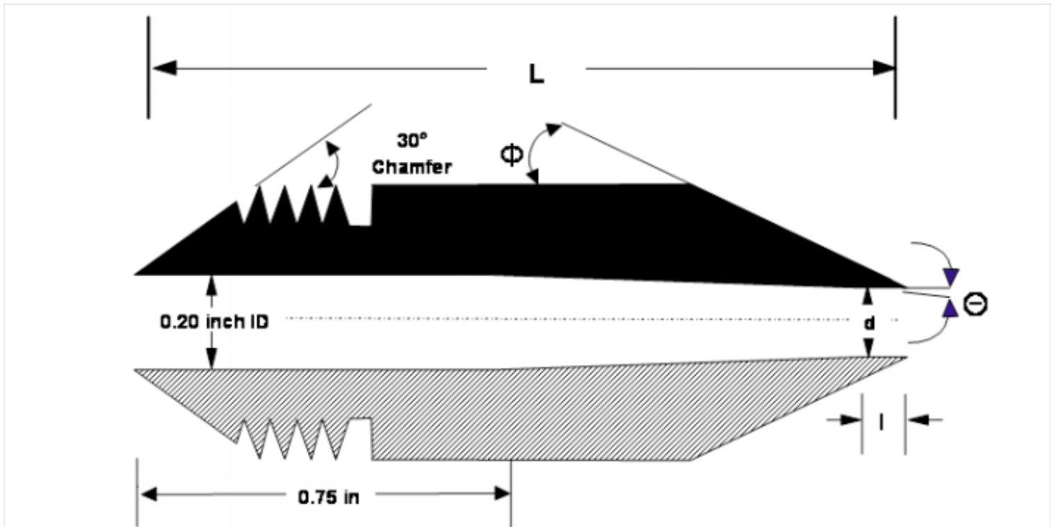
Figure 3. Nozzle Design Specifications for PM 10 Cyclone
