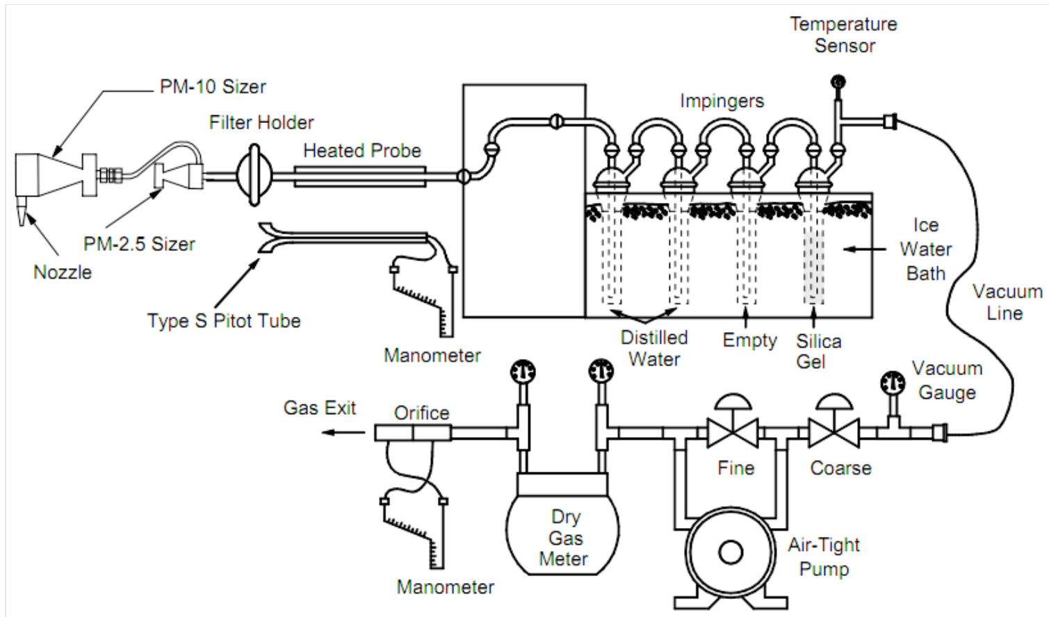
Figure 1. In-stack PM 10 and PM 2.5 Sampling Train
