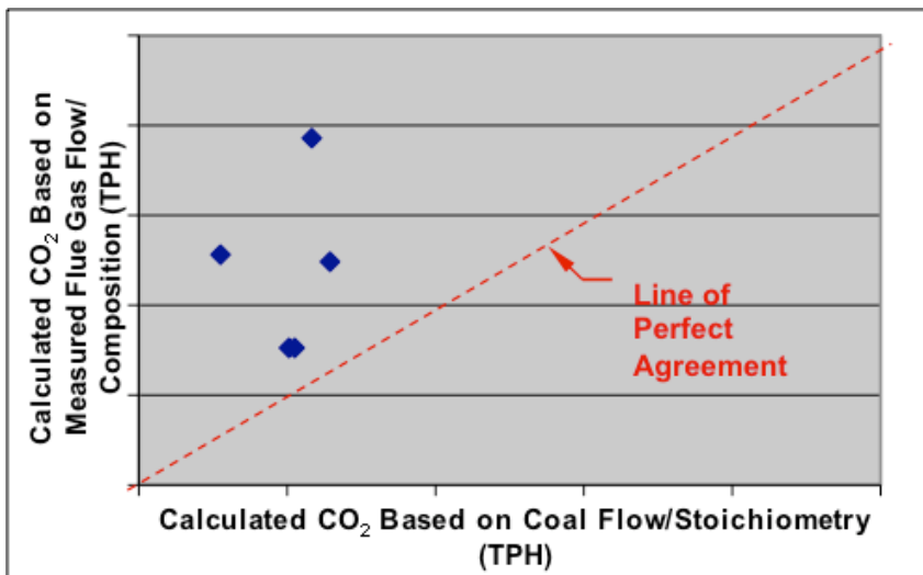
Figure 1. Comparison of calculated vs. measured CO 2 from Plant #1
